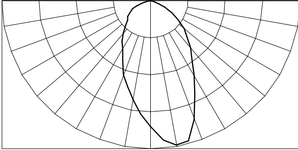
Maximum Candela = 1033.04 Located At Horizontal Angle = 10, Vertical Angle = 10 # 1 - Vertical Plane Through Horizontal Angles (0 - 180)
