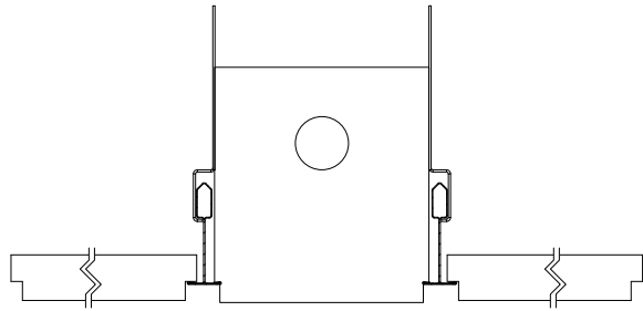
TT9 - 9/16 TEGULAR
