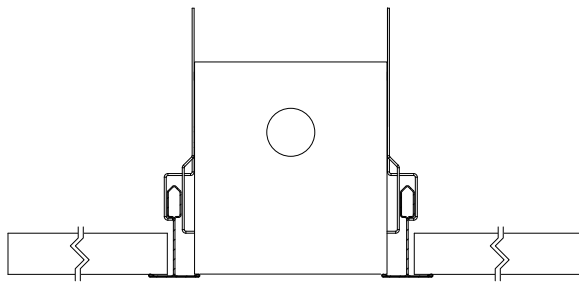
LT15 - 15/16 LAY-IN
